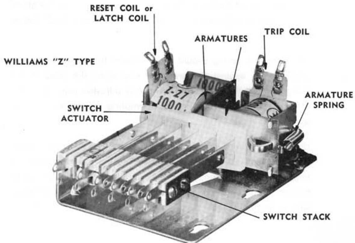
INTERLOCK RELAYS
